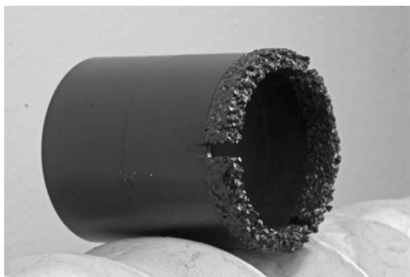
Fig. 4. Crushed carbide rock-coring bit.
