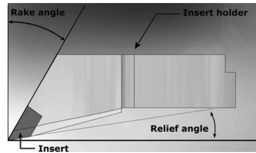
Fig. 3. Koci drill cutter assembly showing rake and relief angles.
