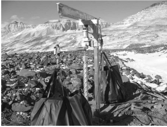
Fig. 1. Koci drill rig in Beacon Valley.
