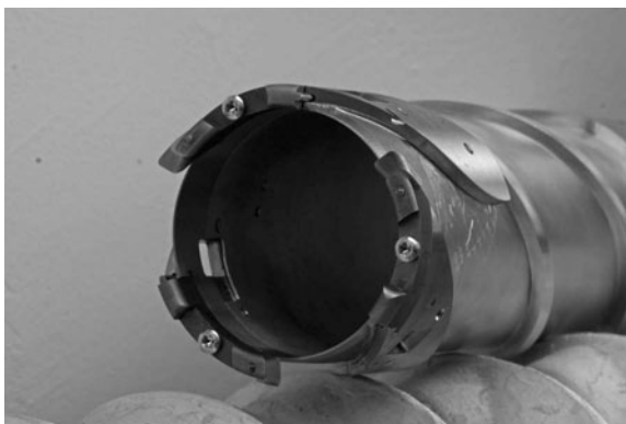
Fig. 2. Koci drill 3 cutter core head.
