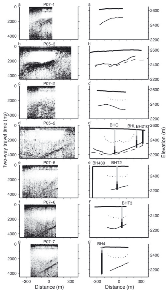
Fig. 3. (a–g) Radargrams recorded at 40 MHz, displayed in the twt domain. (a'–g') Ice geometry and schematic interpretation of profiles (a–g) in the depth domain, converted to elevation (m a.s.l.): surface topography (thick curves), bedrock topography (deduced from 40 MHz data: thin curves; 1–5 MHz data (only (b') and (d')): dashed curves), and depth of cold–temperate transition surface (CTS) 40 MHz data, dotted curves). Vertical lines (d'–g') show projected location of boreholes onto the nearest radar profile along tentative flowlines; thin black line indicates borehole extent without thermistors; bold lines indicate thermistor chains; and line fillings indicate temperatures: below pmp (light grey); thermistor gap containing CTS (grey, see Table 1); and temperate ice (black). Ice flow is into the plane.
