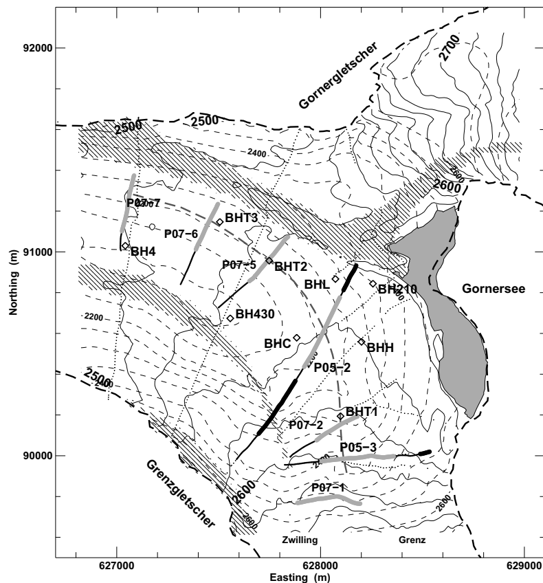
Fig. 1. Overview of study area at confluence of Gorner- and Grenz glaciers with the Gornersee (solid grey area): surface elevation with 20 m contour lines (thin solid), bedrock elevation with 50 m contour lines (dashed), borehole locations (labelled diamonds), low-frequency radar profiles (dotted lines) and extent of medial moraines at surface (hatched). Along the 40 MHz radar profiles (P05-2 to P07-7, semi-bold lines) the presence of the low backscatter at 60 m depth is indicated as a grey bold line, the presence of clutter as a black bold line. The semi-bold dashed grey line indicates a tentative flowline (BHT4-BHT2-BH3), the semi-bold dashed black line the glacier boundary.
