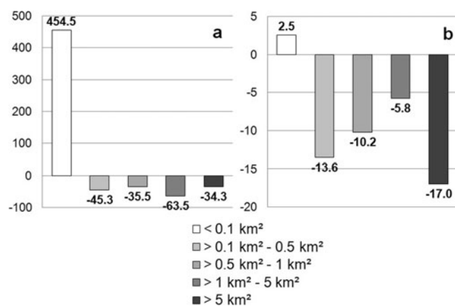
Fig. 3. Glacier number and area size change by different classes as (a) percentage change of the total number, and (b) total area ( \text{km}^2 ) between 1983 and 2006.
