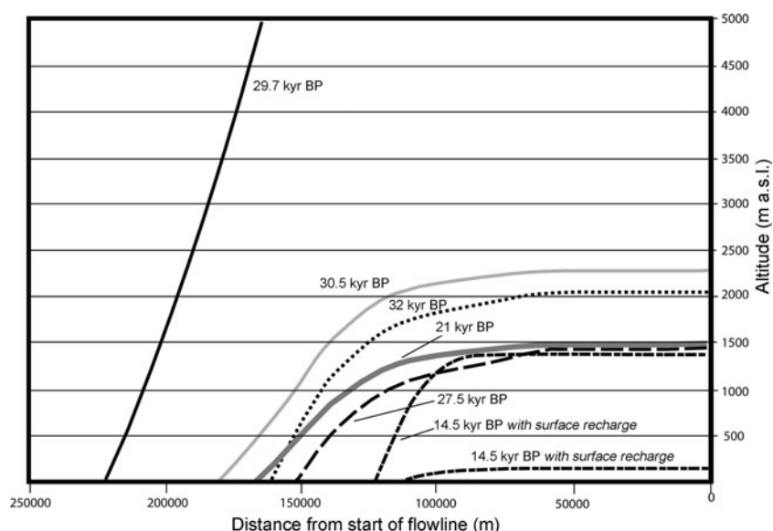
Fig. 3. Profiles of the potentiometric surface from the two-layer model for each simulated ice position.
