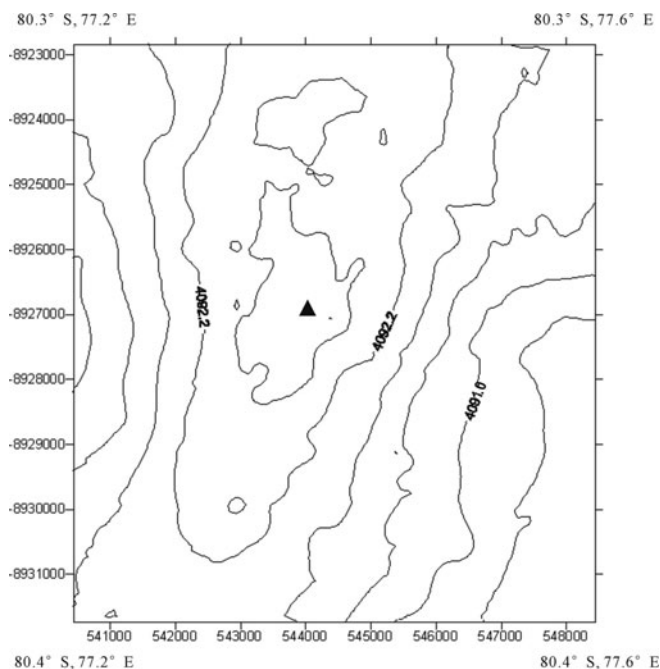
Fig. 1. Dome A surface topographic map based on GPS data from the 21st CHINARE. Heights are relative to the WGS84 ellipsoid. Contour interval is 0.40 m. The black triangle indicates the position of the summit of Dome A.
