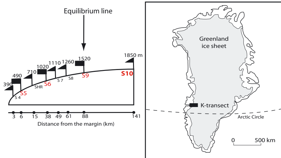
Fig. 4. The location of the K-transect in the ablation area of the West Greenland ice sheet, together with a cross section showing the names, heights and distance from the ice edge for each site. The locations of the AWSs are marked red.
