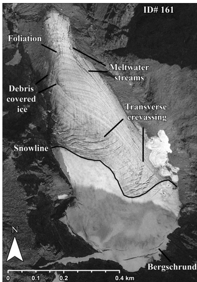
Fig. 4. Aerial photograph of an actively flowing mountain glacier near Ryan's Bay (52.53°N 64.00°W) in the Torngat Mountains. The image is labeled with examples of glaciological features that categorize glacier flow.
